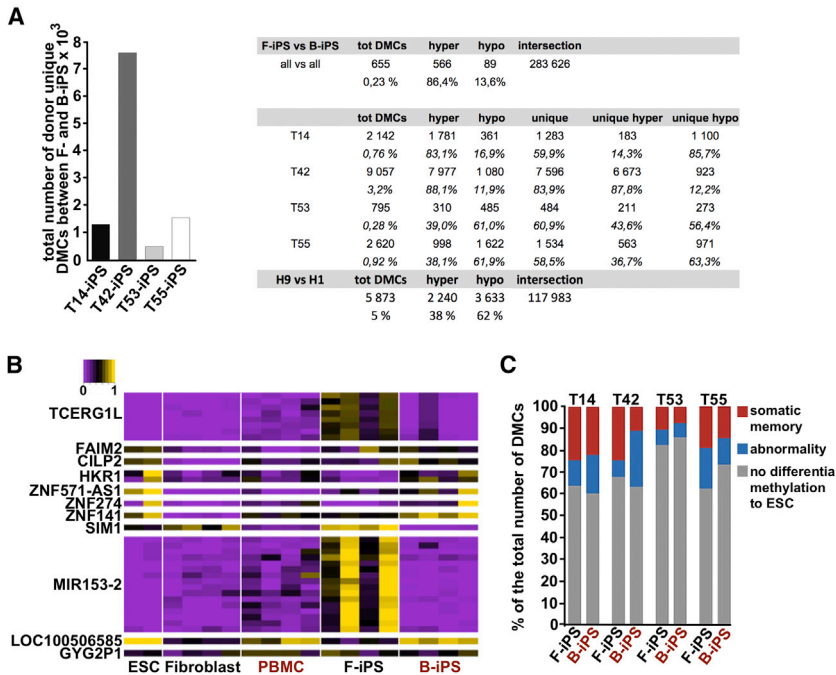
Figure 2. Methyloomic Analyses Demonstrate Minimal Contribution of Source-Cell-Specific Differences to iPSC Variability
